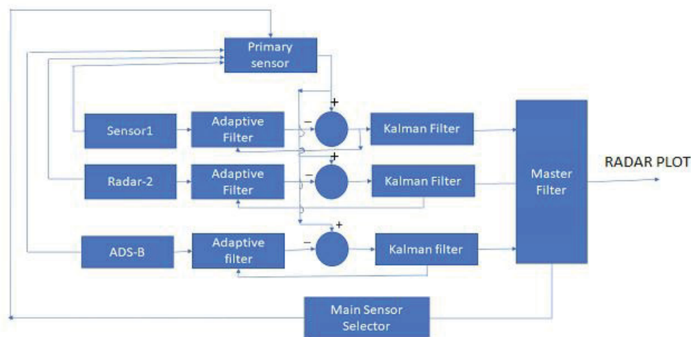
Figure 3: Adaptive filter with Kalman filter block diagram.
