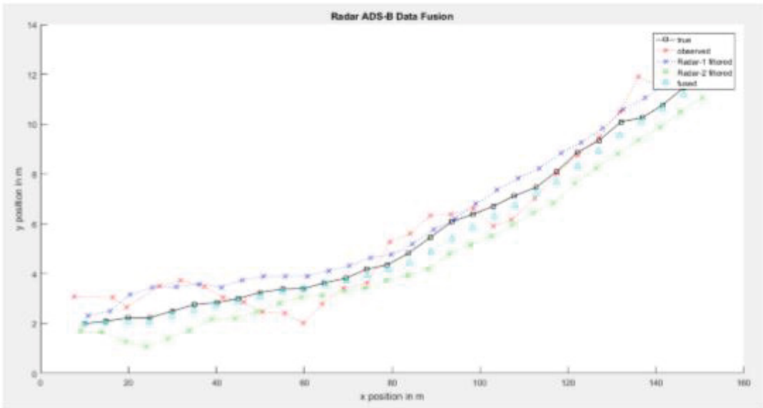
Figure 8: Radar, ADS-B and fusion results.
