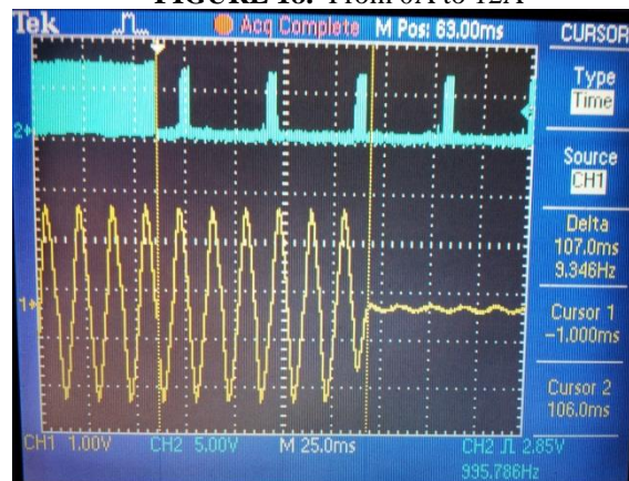
FIGURE 19. From 12A to 0A
