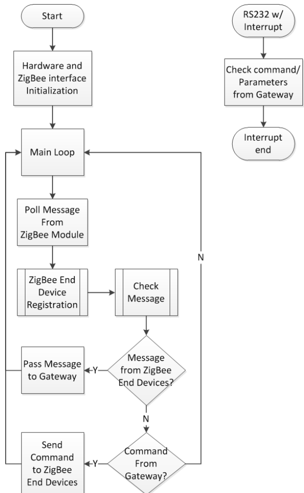
FIGURE 13. ZigBee coordinator firmware flow
