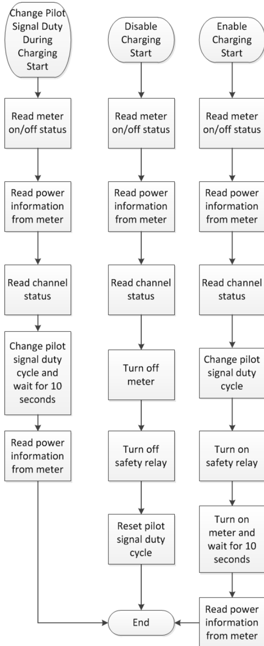
FIGURE 14. Server operation flow
