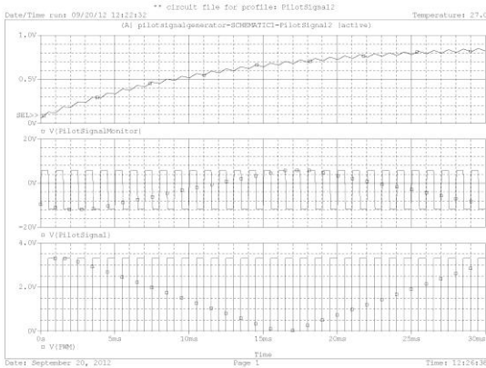
FIGURE 11. Pilot signal peripheral circuit simulation with EV. (From bottom to top: (1)PWM from MSP430,(2)Pilot signal,(3)signal at pilot signal monitor)
