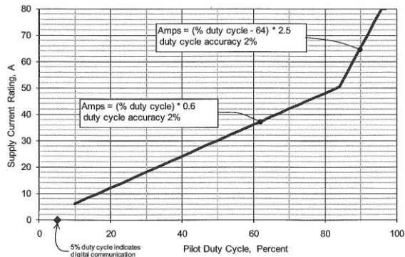
FIGURE 5. Supply current v.s. pilot duty cycle[12].
