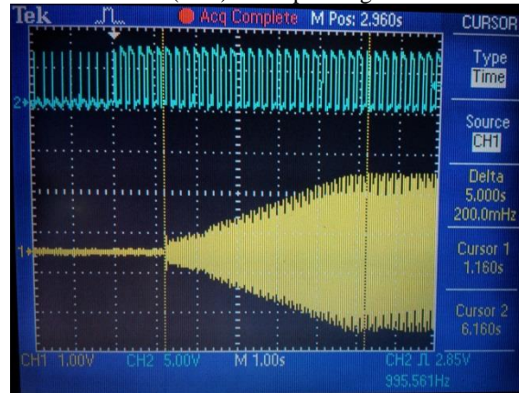
FIGURE 18. From 0A to 12A
