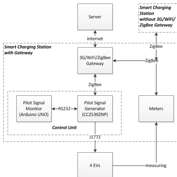
FIGURE 2. Details of smart charging station
