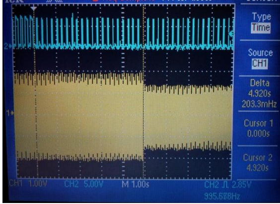
FIGURE 21. From 12A to 8A
