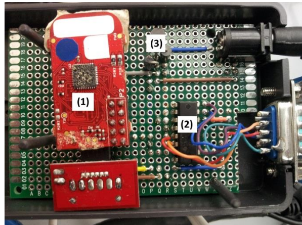
FIGURE 12. ZigBee coordinator implementation: (1) ZigBee CC2530ZNP (2) MAX3232 (3) Regulator
