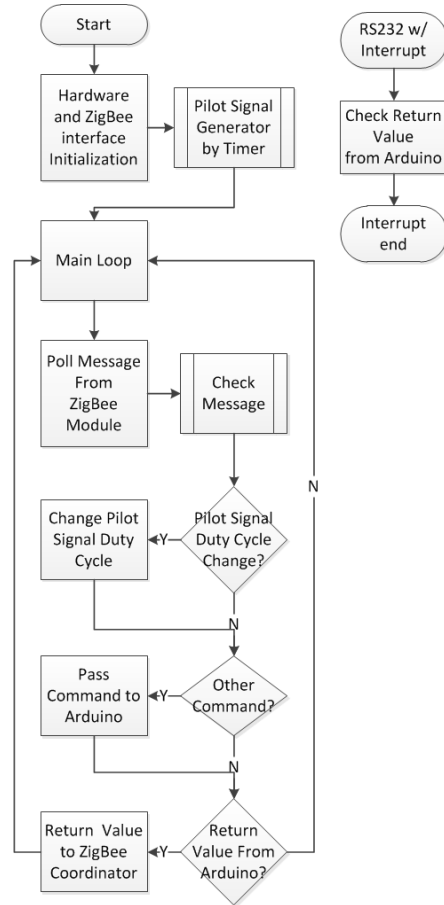
FIGURE 7. Firmware flow of MSP430 of CC2530ZNP as the ZigBee end device (pilot signal generator)
