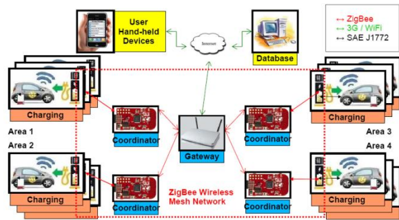
FIGURE 1. Smart charging infrastructure
