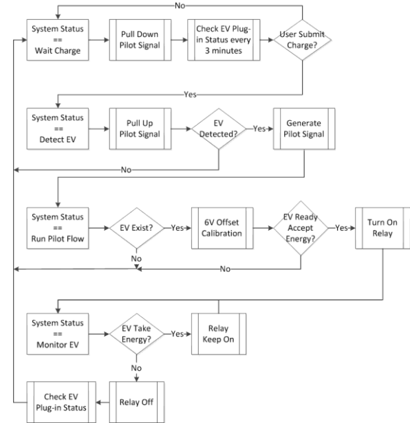
FIGURE 9. State machine flow chart.
