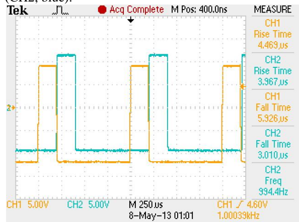
FIGURE 17. Comparison between our pilot signal and original pilot signal
