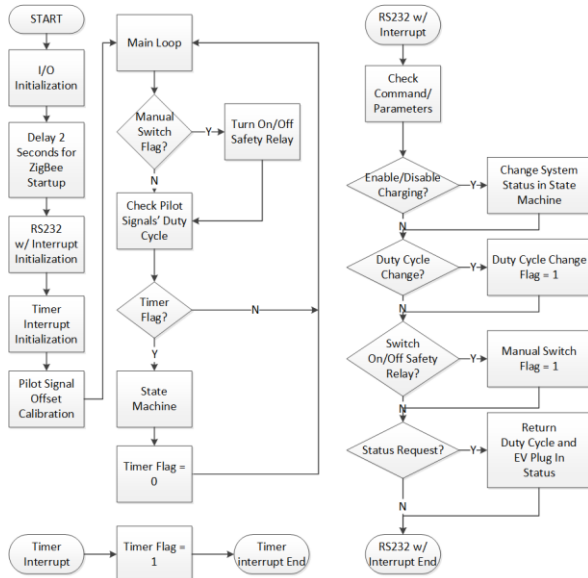
FIGURE 8. Pilot signal monitor firmware flow chart.
