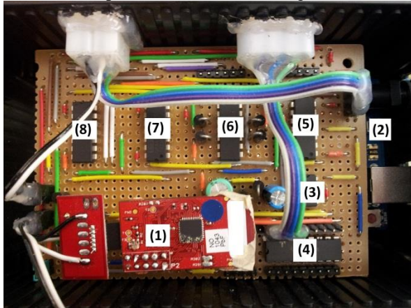
FIGURE 6. Realization of the control unit: (1)pilot signal generator (2)pilot signal monitor (3)555 counter (4)relay driver (5)Schmitt trigger (6)unit gain buffer (7)inverting amplifier (8)inverting LPF.
