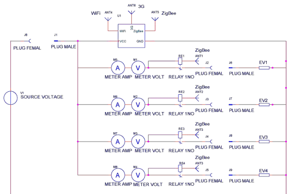
FIGURE 3. Schematics of metering system
