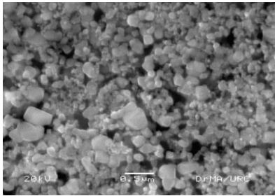
FIGURE 2.(b) Scanning electron image of ZnO-SnO 2 nanocomposite film
