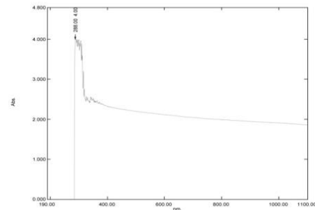
FIGURE. 3.(b) The optical absorption spectra of ZnO-SnO 2 nanocomposite film
