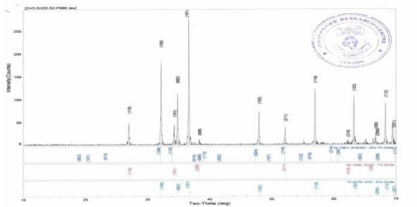
FIGURE 1.(b) XRD profile of ZnO-SnO 2 nanocomposite film
