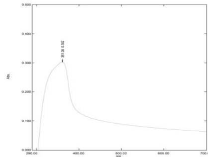
FIGURE 3.(a) The optical absorption spectra of ZnO nanorod film
