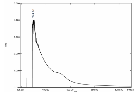
FIGURE. 3.(c) The optical absorption spectra of onion skin natural dye
