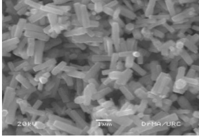
FIGURE 2.(a) Scanning electron image of ZnO nanorod film
