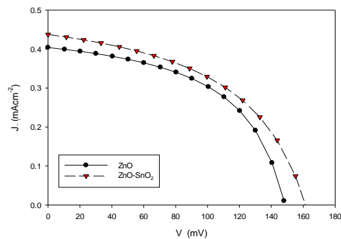
FIGURE. 4. J-V characteristic curve for ZnO and ZnO-SnO 2 nanocomposite electrode DSSC
