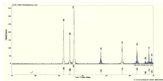
FIGURE 1. (a) XRD profile of ZnO nanorod film
